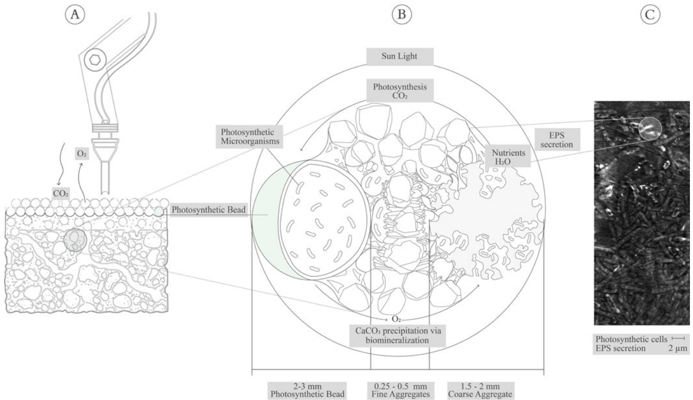
Figure 6. Proposed multiscale workflow toward self-sustaining, long-term viable architectures, integrating microbial, material and fabrication scales. (A) 3D printing of a functionally graded biocemented component, utilizing spatially varied density to optimize both biological and architectural performance. (B) Internal metabolic loops and interactions between PhotoBeads, fine sand aggregates and coarse sand aggregates. The matrix is bound by hydrogel and biogenic EPS, culminating in biocementation via \text{CaCO}_3 precipitation. (C) SEM image of the biofilm formed by photosynthetic microorganisms.
