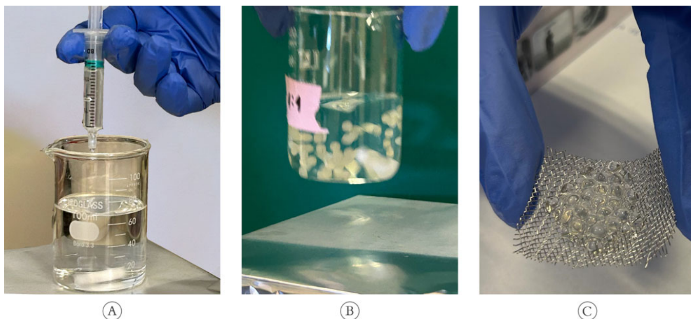
Figure 2. Development and optimization of abiotic hydrogel beads, establishing the material baseline for future photosynthetic cell encapsulation. (A) Extrusion of the hydrogel precursor via the syringe. (B) Ionic crosslinking within a calcium bath. (C) Fully crosslinked abiotic beads on a grid.
