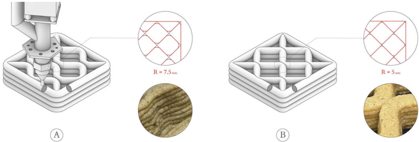
Figure 8. Toolpath-material optimization. (A) Due to a higher toolpath radius, material drag increased while overall shape fidelity reduced, resulting in print failure. (B) Smaller toolpath radius increased shape fidelity and buildability, resulting in comparable total print height without collapse.
