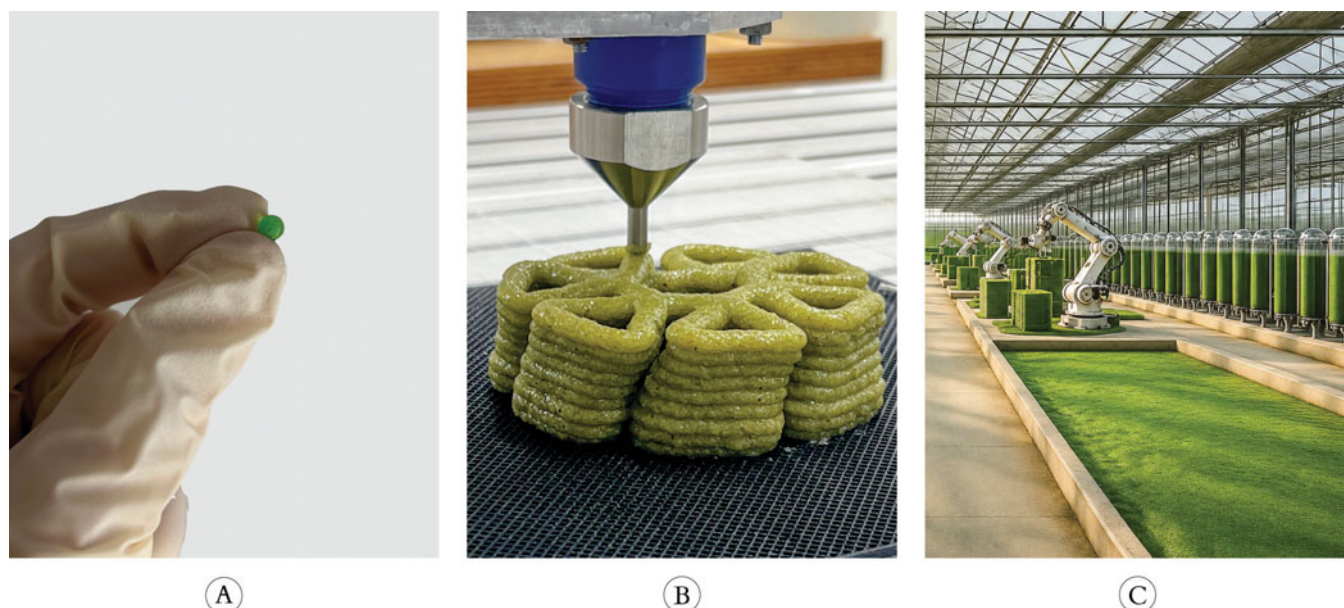
Figure 1. Representative images of the three case studies. (A) Case Study 1: hydrogel-based encapsulation strategy for sustaining photosynthetic bead viability and long-term durability. (B) Case Study 2: robotic additive manufacturing of microbe-based building materials. (C) Case Study 3: conceptual model of building materials agriculture, depicting the co-site of cultivation and fabrication systems (generated using AI tools).
