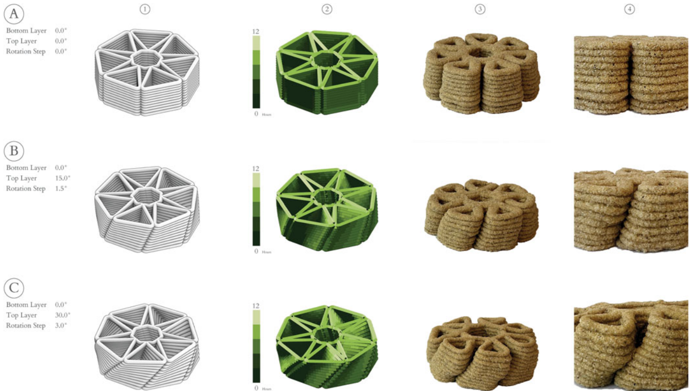
Figure 9. Biologically informed design catalog. The figure compares three toolpath variations, examining the relationship between geometric modification for enhanced light exposure (1&2) and corresponding printing performance (3) in terms of buildability, slumping and shape fidelity (4). (A) Extruded component with no rotation. (B) Extruded component with 1.5° rotational increase. (C) Extruded component with 3.0° rotational increase.
