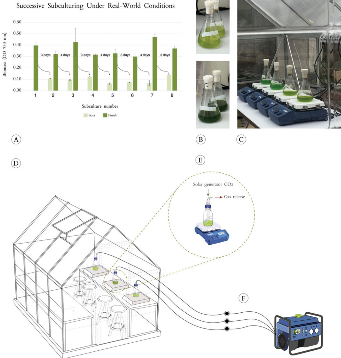
Figure 11. (A) Biomass accumulation (OD 750 ) during successive subculturing, demonstrating culture stability under living lab conditions. (B) Representative culture at the beginning of a generation (light green) compared to the same culture after 3–4 days of growth (dark green). (C) Experimental configuration of multiple photosynthetic strains cultivated within the living lab. (D) Schematic representation of the living lab system. (E) Diagram of the gas delivery configuration, illustrating inlet and outlet connections supplying generator exhaust to each culture vessel (F).
